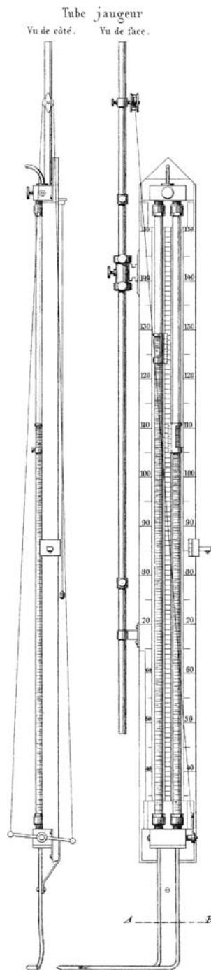
Fig. 7 The Pitot tube design used by Darcy in his 1856 report (Darcy 1856, Plate 23, Fig. 14)
