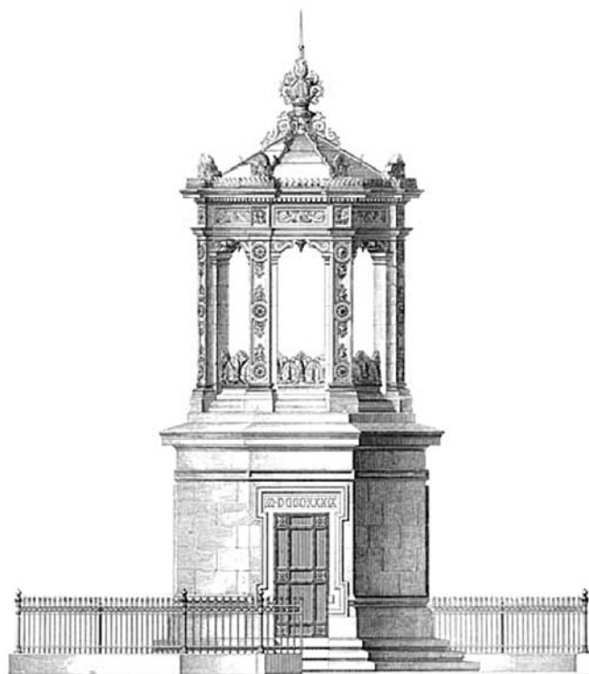
Fig. 4 Darcy's design of the tower at Porte Guillaume reservoir (Darcy 1856, Plate 9). The tower and reservoir are still standing today
