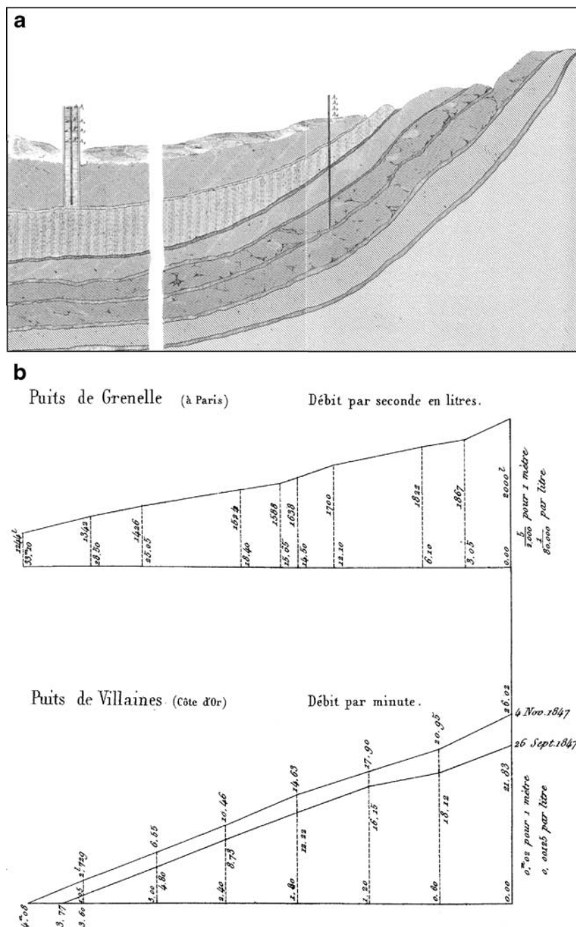
Fig. 6 Artesian well flow a Darcy's schematic of artesian flow measurements showing a geologic cross-section, and b flow rate measured as a function of the discharge elevation at two sites. A clear linear trend was observed in these and other data sets. (Darcy 1856, Plate 22)
